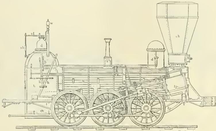
MILLHOLLAND'S PHILADELPHIA. FIG. 75.
